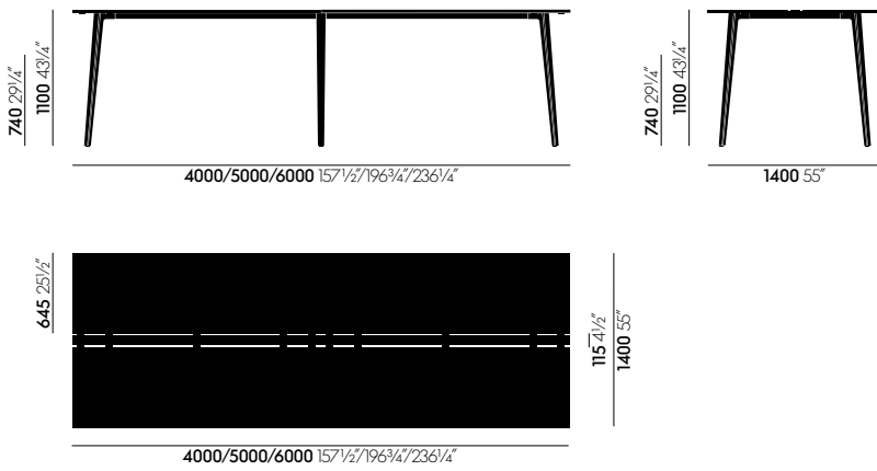
Joyn 2 Touchdown table 400/500/600 x 140 cm, table height 74/110 cm
