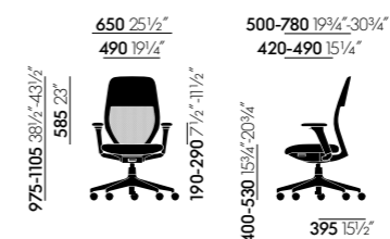
ACX Light with height-adjustable armrests
