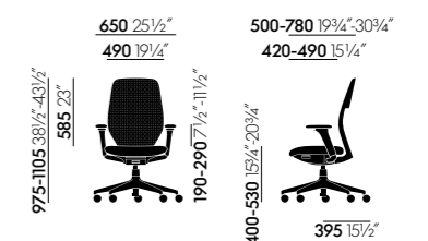
ACX Soft with height-adjustable armrests
