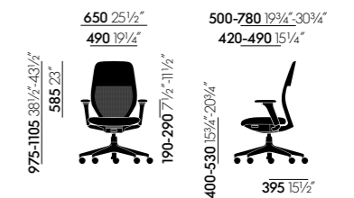
ACX Mesh with height-adjustable armrests
