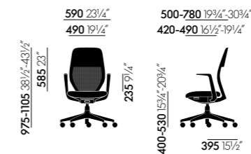
ACX Mesh with fixed armrests
