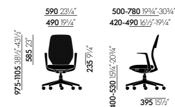
ACX Soft with fixed armrests
